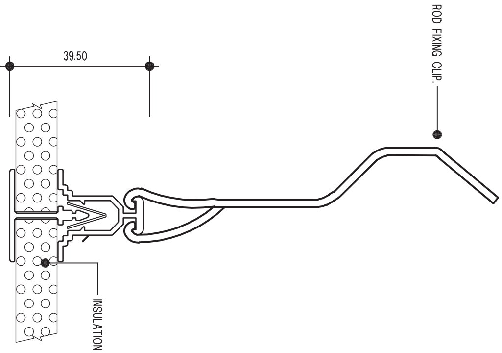
(SIDE ON VIEW OF STARTER BAR.)
